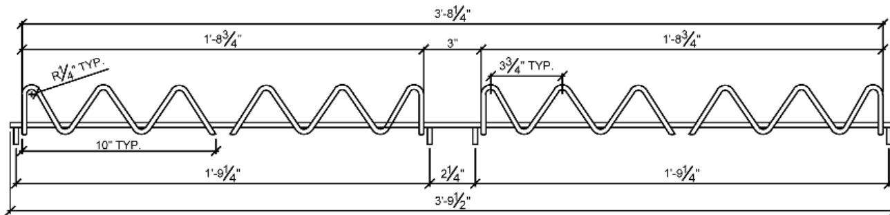
ELEVATION VIEW
